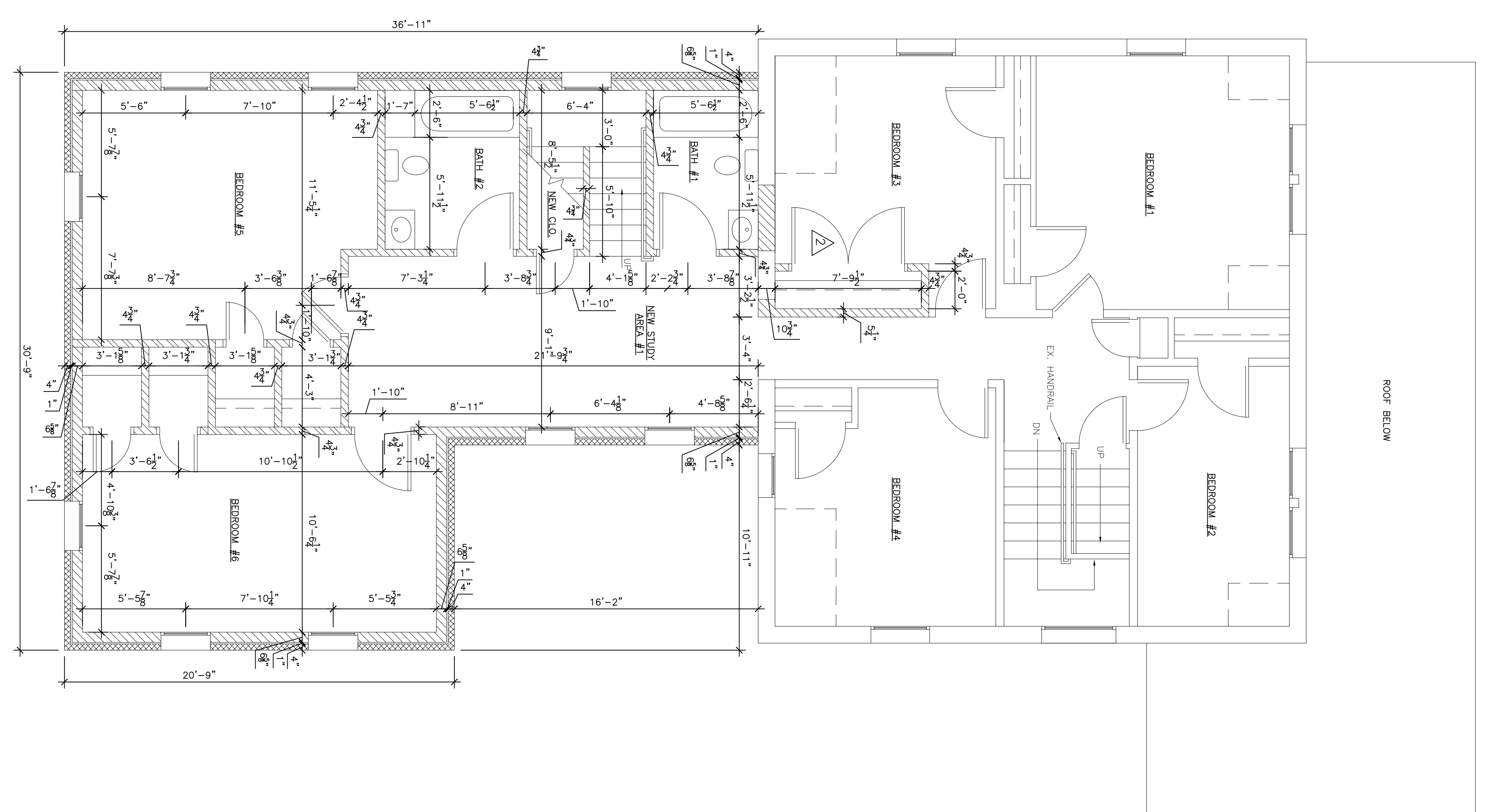
PROPOSED SECOND FLOOR DIMENSION PLAN SCALE: 1/4" = 1'-0"
