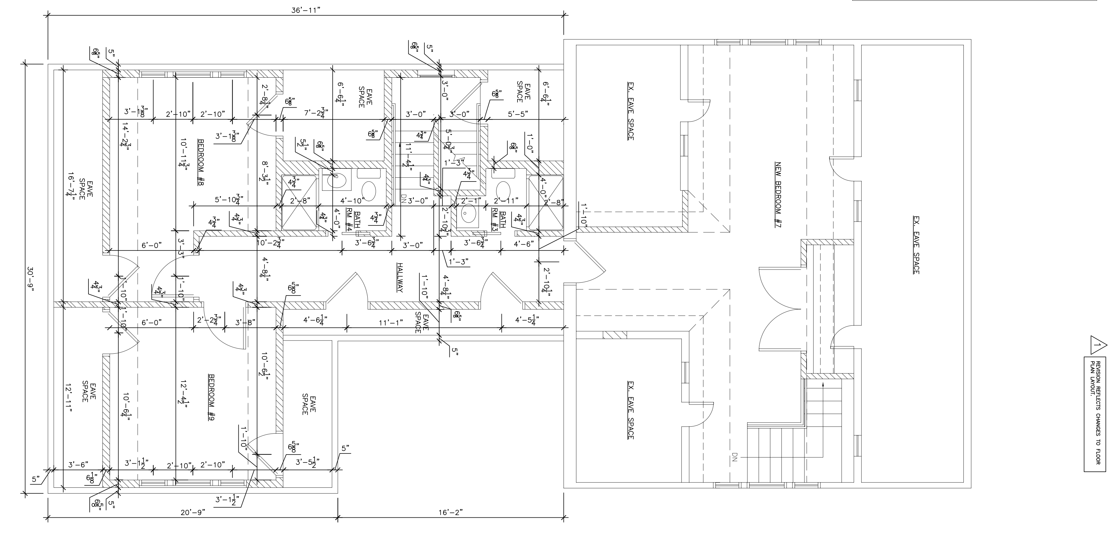
PROPOSED THIRD FLOOR DIMENSION PLAN SCALE: 1/4" = 1'-0"
